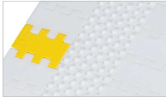
M2514 Nub Top
